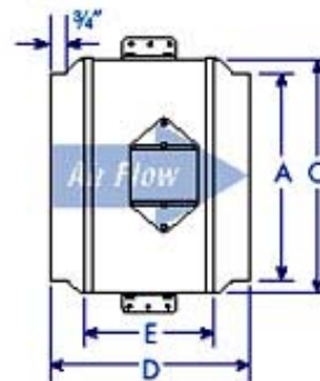
Side View - FKD8XL
