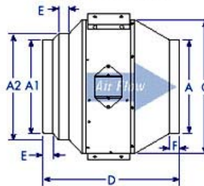
Side View - FKD12XL
