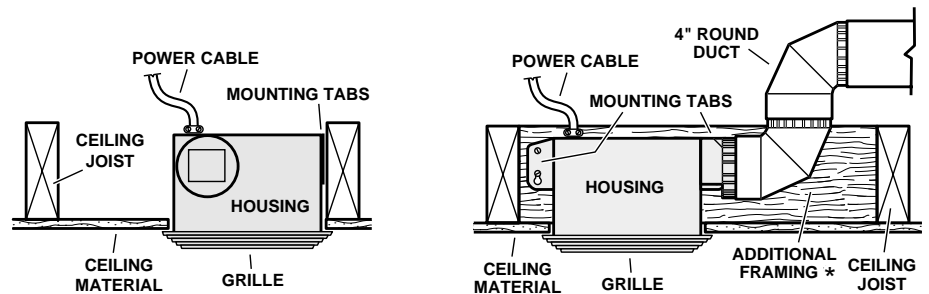
HOUSING MOUNTED DIRECTLY TO JOIST 2x6 (or larger)
