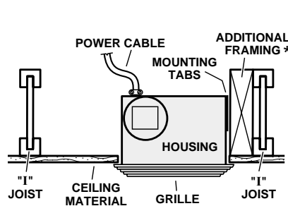
HOUSING MOUNTED TO "1" JOIST
